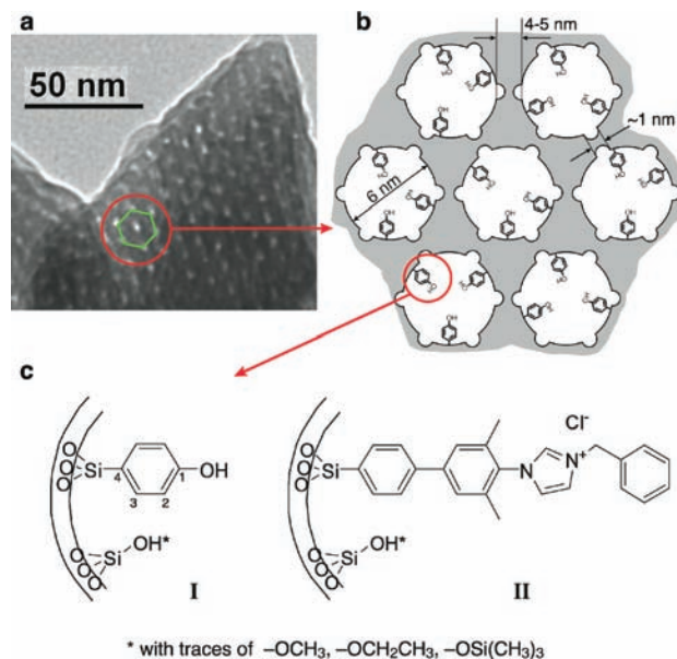
Figure 1. (a) Transmission electronic microscopy image of the nanoporous silica material. (b) Schematic representation of the pore [mesopores (6 nm diameter) are shown as circles and micropores (<1 nm diameter) as small half-circles] and channel network with phenol functionalities. The shaded gray area represents the silica bulk. (c) Different covalently incorporated aromatic substrates.
